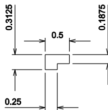
SIDE VIEW 1
